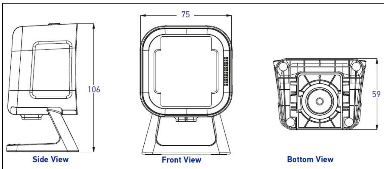
Figure 6. Riser Stand Dimensions
