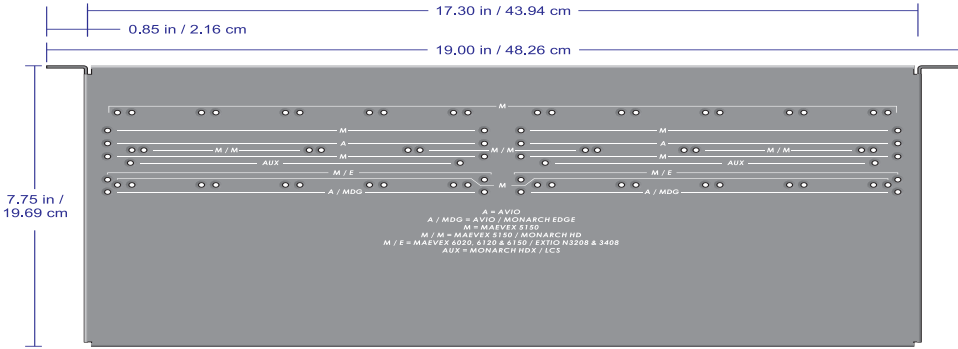
Mounting shelf – Underside
