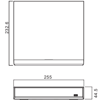
Figure 2-1 Dimensions (Unit:mm)
