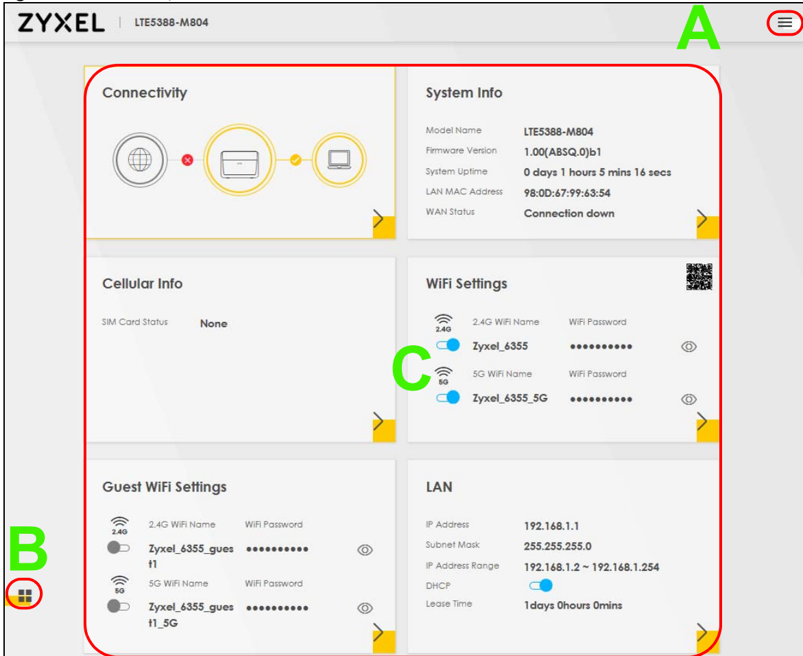
Figure 36 Screen Layout
