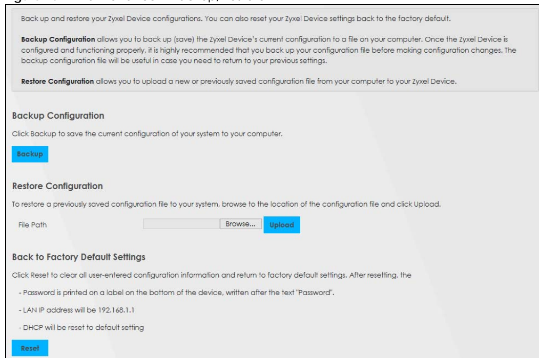
Figure 202 Maintenance > Backup/Restore
