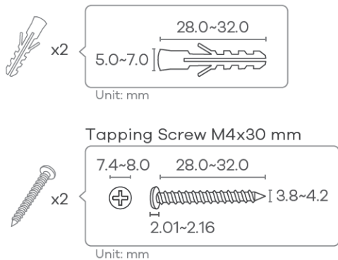
Figure 33 Wall Mounting Screw Specifications
