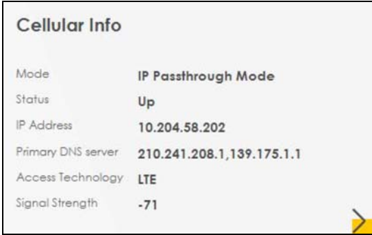
Figure 54 Cellular Info
