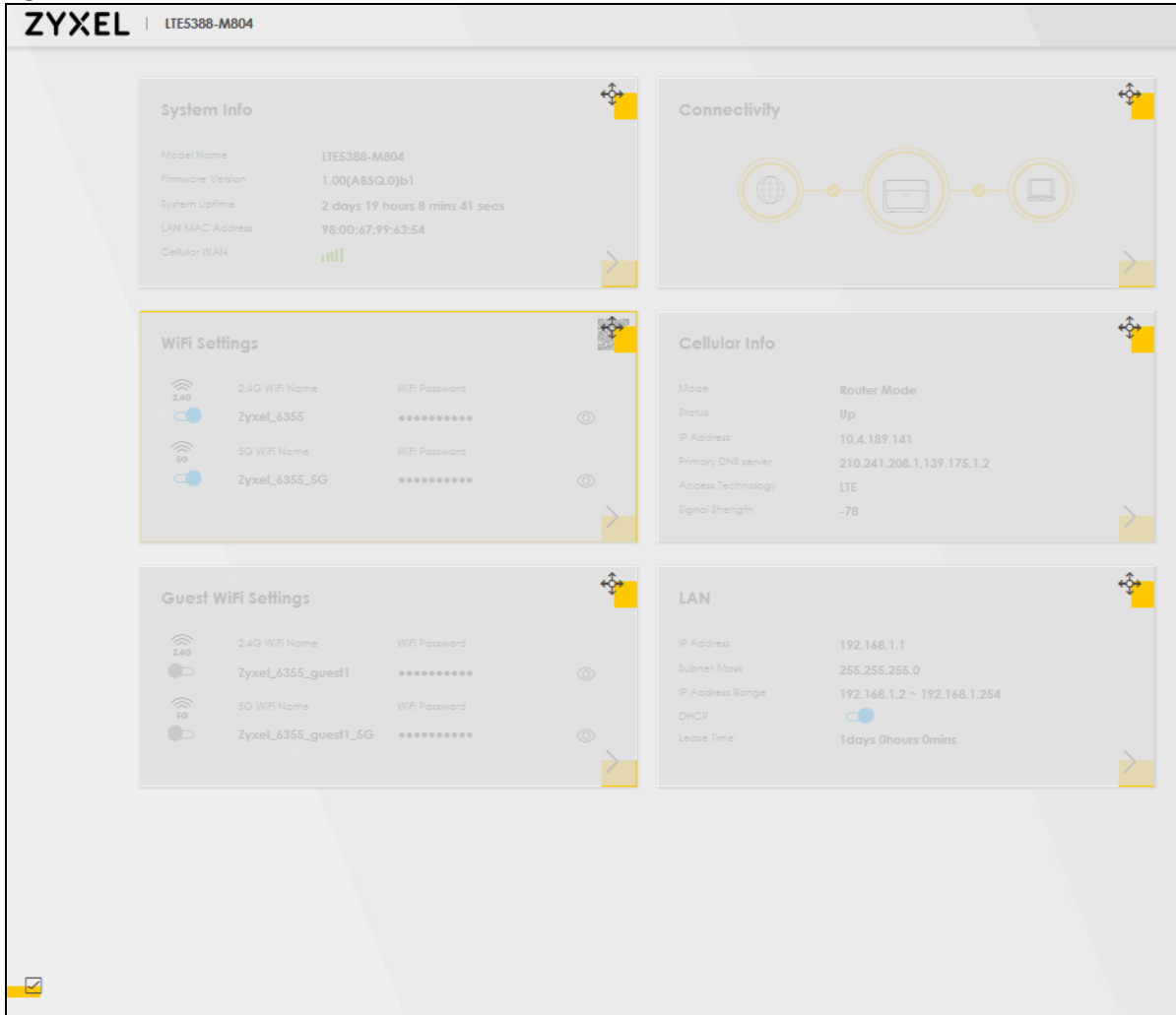
Figure 40 Screen Order
