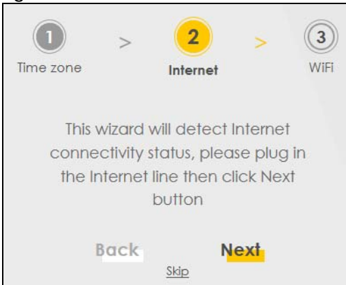
Figure 43 Wizard – Internet
