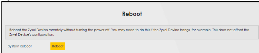
Figure 206 Maintenance > Reboot
