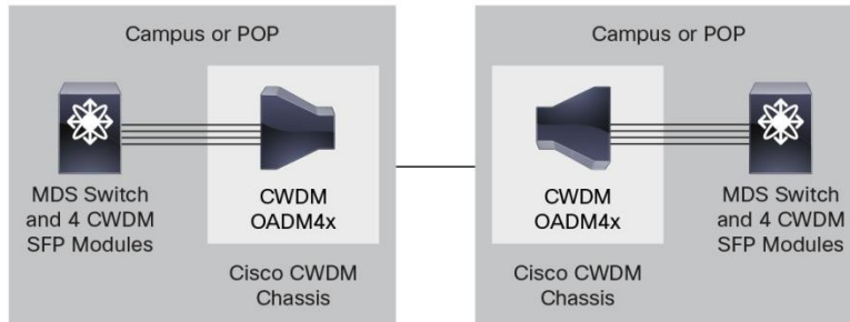
Figure 14. Point-to-Point Architecture (Dual-Fiber Link)
