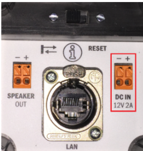
Figure: Power Supply Connection
