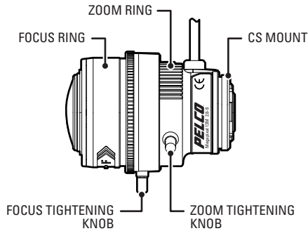
Figure 2. Adjustment Controls (13M2.8-8 Shown)
