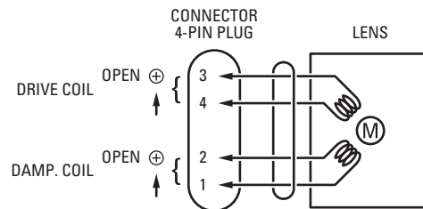
Figure 1. Lens and Connector Wiring
