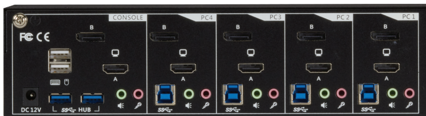
FIGURE 3-1. KV6224DPH – REAR VIEW
