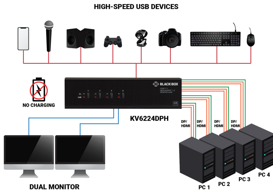
FIGURE 3-2. CONNECTION ILLUSTRATION
