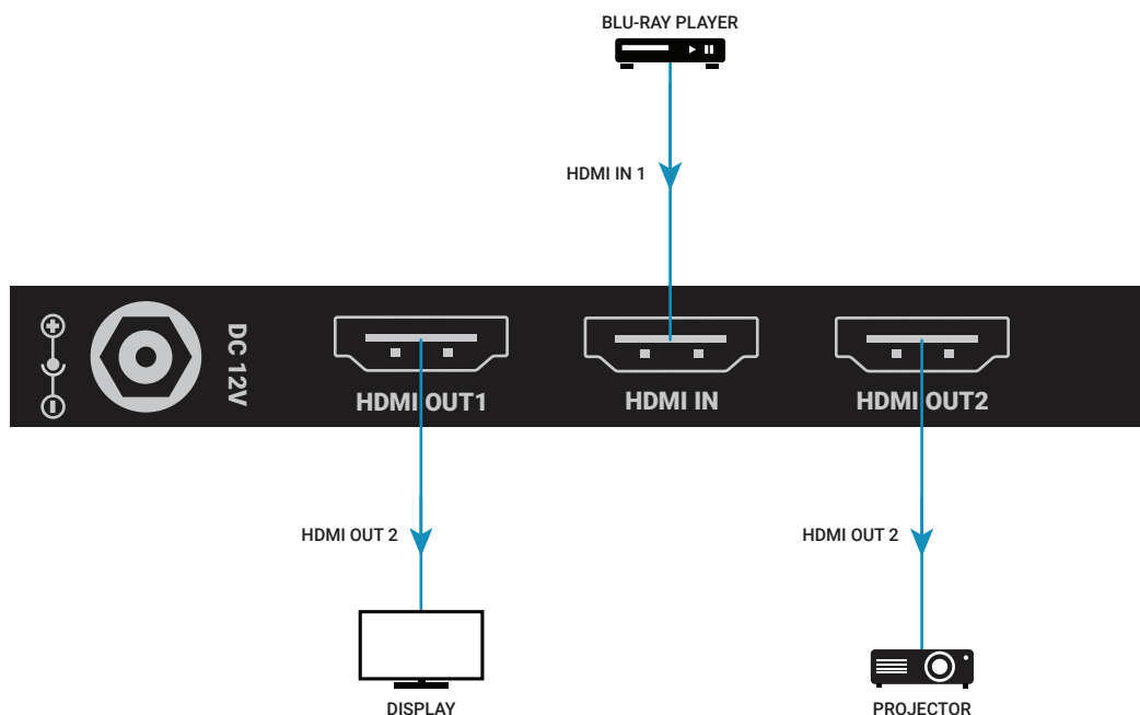
FIGURE 3-1. TYPICAL APPLICATION
