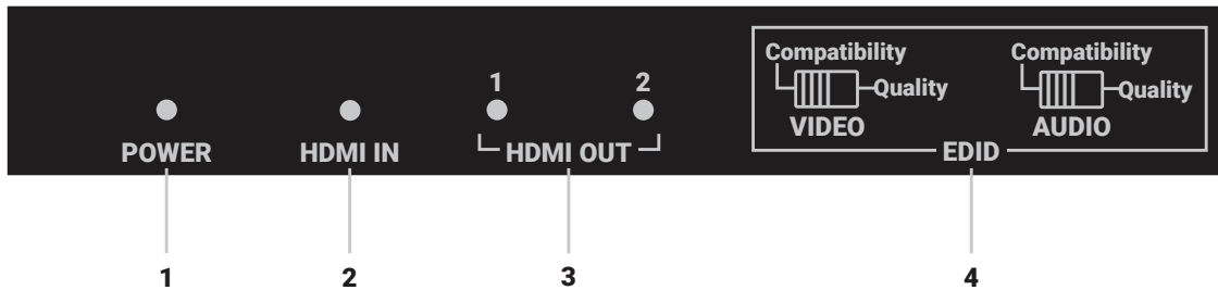
FIGURE 2-1. SPLITTER FRONT PANEL
