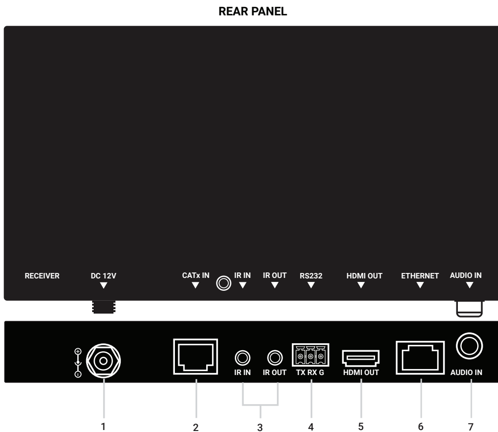
FIGURE 2-4. RECEIVER BACK PANEL
