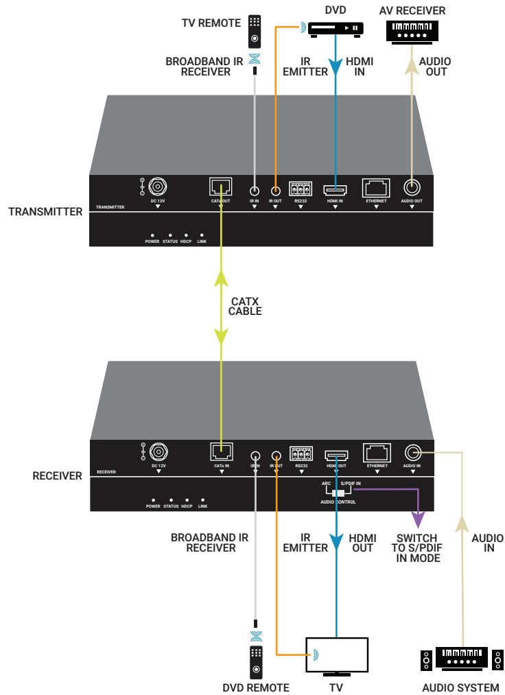
FIGURE 3-2. CONFIGURE S/PDIF
