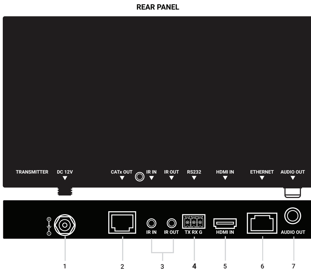
FIGURE 2-2. TRANSMITTER TOP AND BACK PANEL
