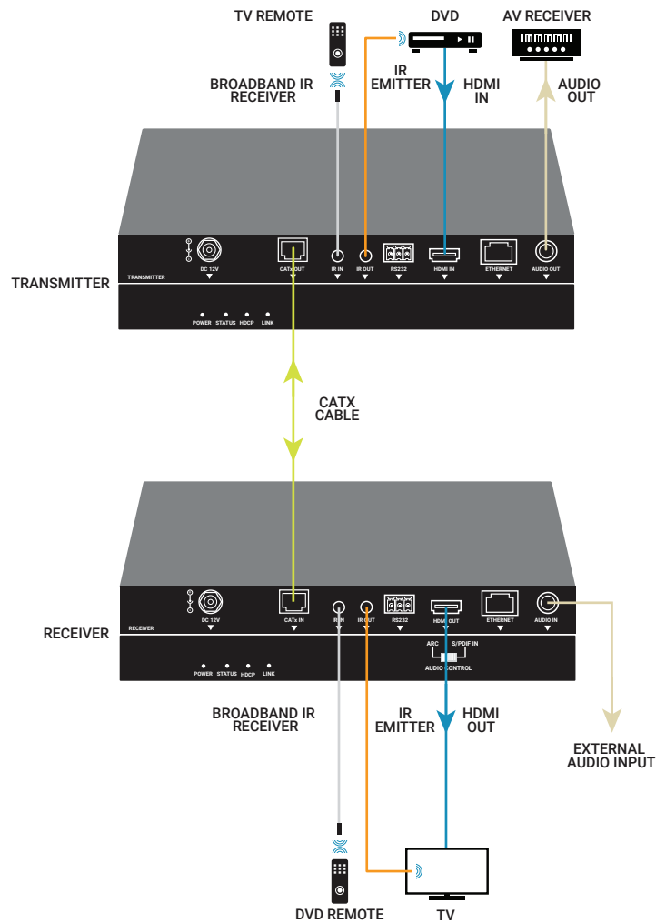
FIGURE 3-1. CONFIGURE ARC CHANNEL
