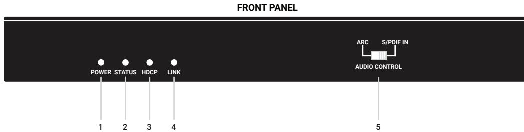
FIGURE 2-3. RECEIVER FRONT PANEL
