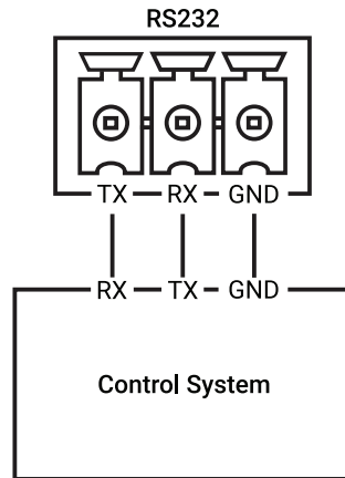
FIGURE 5-1. RS-232 PINOUT
