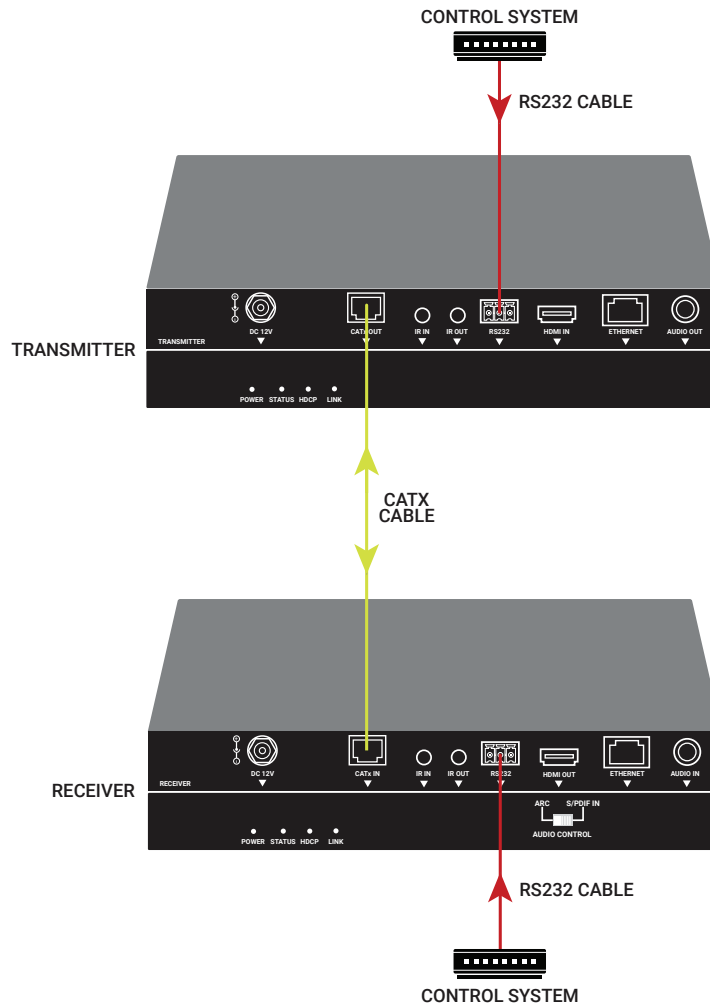
FIGURE 5-2. RS-232 PASSTHROUGH
