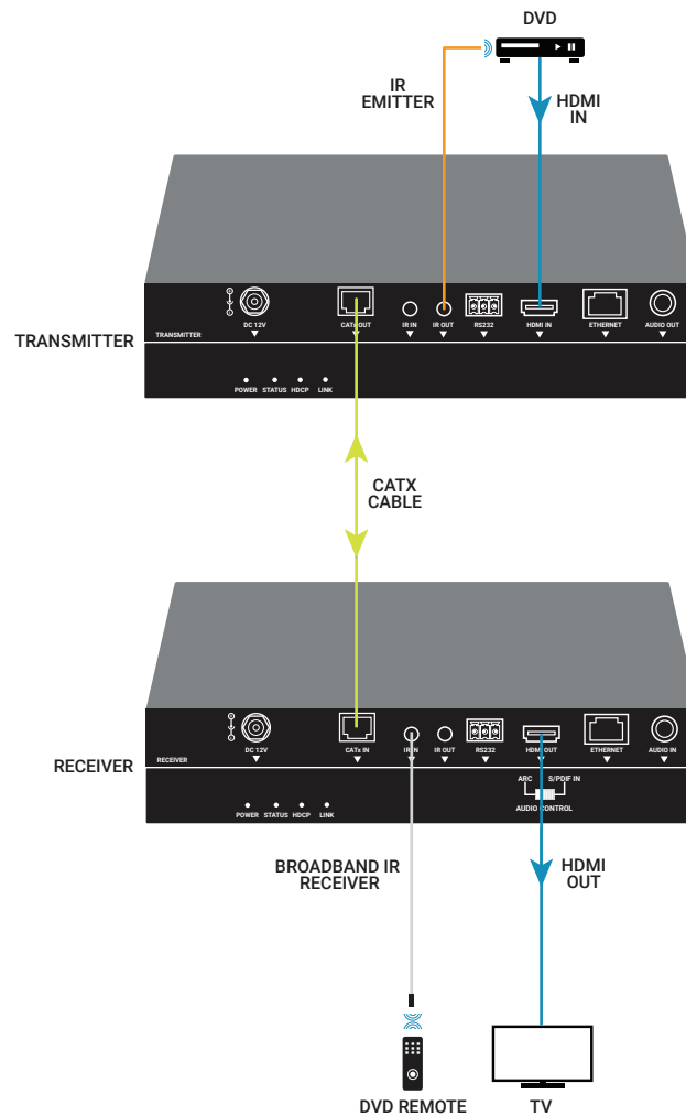
FIGURE 4-2. CONTROL THE SOURCE
