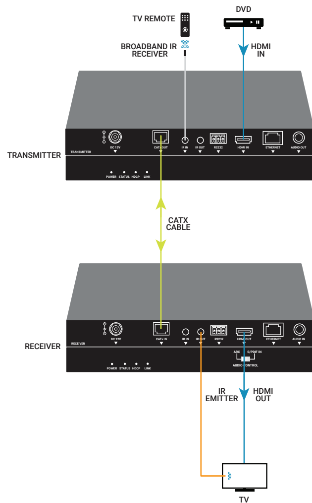
FIGURE 4-1. CONTROL THE DISPLAY
