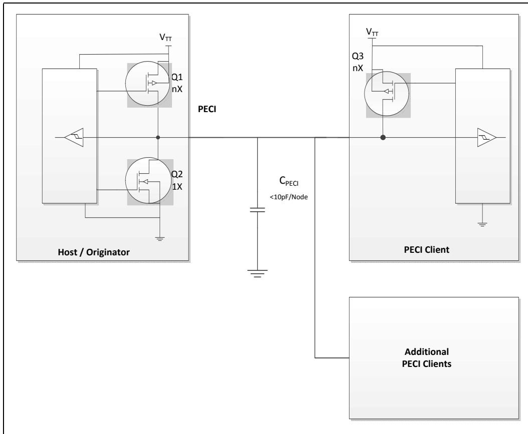
Figure 2-9. Example for PECl Host-Clients Connection
