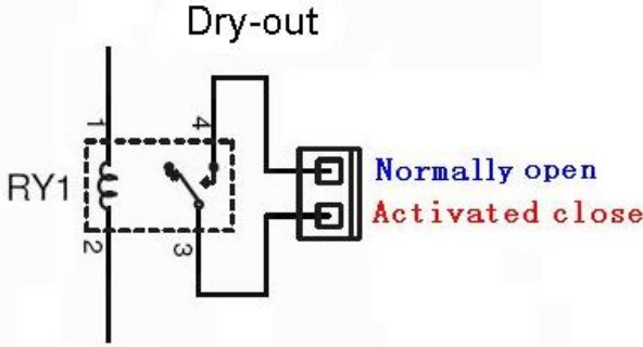
Dry out contact schematic
