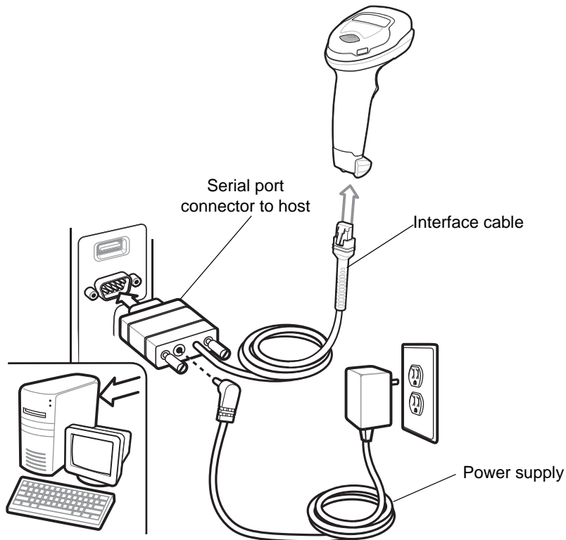
Figure 8-1 RS-232 Connection
