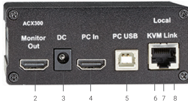
FIGURE 2-2. BACK PANEL OF THE LOCAL EXTENDER
